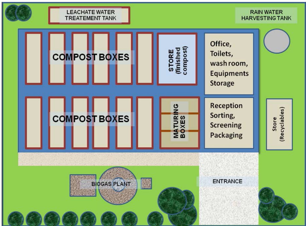
Schematic Layout of Box-Type Compost Plant IRR Design
