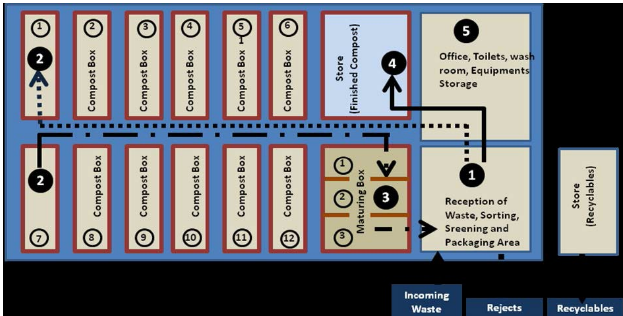
Schematic Layout of Box-Type Compost Plant IRR Design
